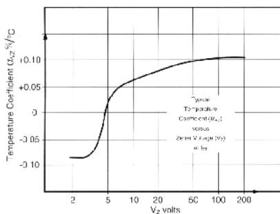
Figure 1. Temperature Coefficient vs Zener Voltage
