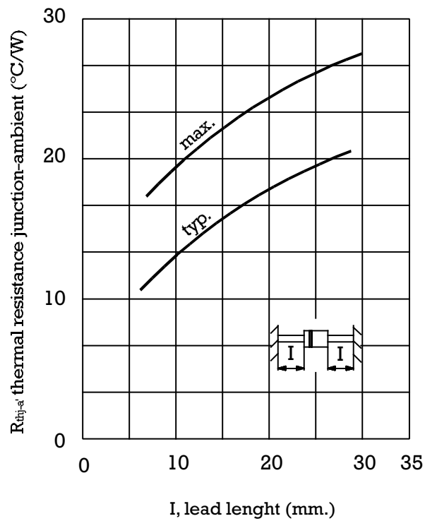
THERMAL RESISTANCE
