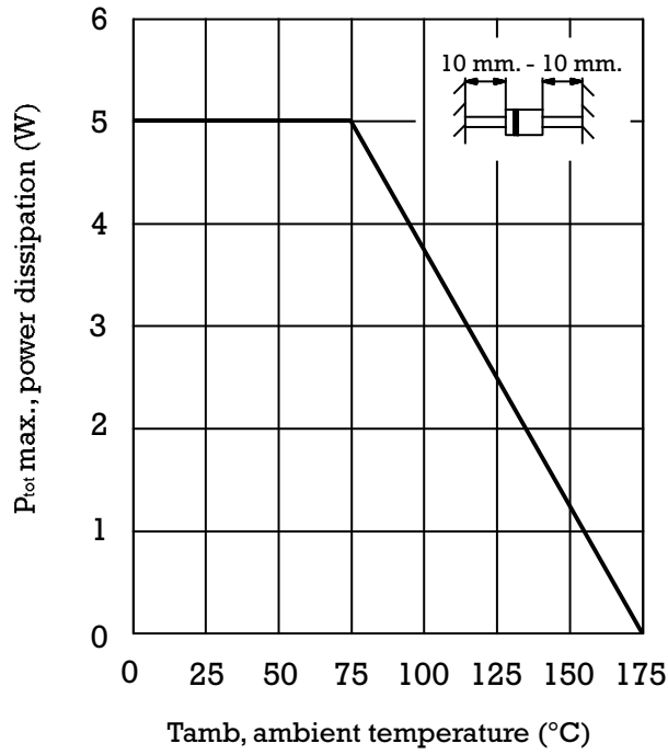
THERMAL RESISTANCE
