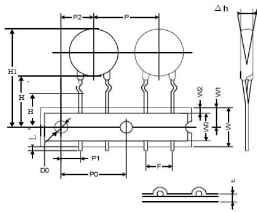
Crimped Leads (5D,7D,10D)
