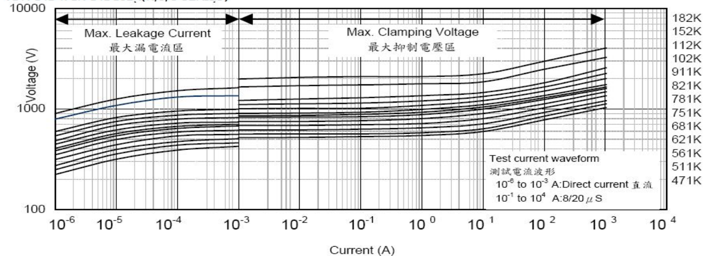
VDR-14D471K-14D182K(N/J/S SERIES)
