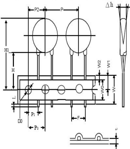
Straight Leads (10D,14D,20D)
