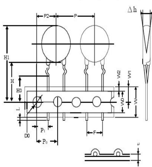
Crimped Leads (10D,14D,20D)
