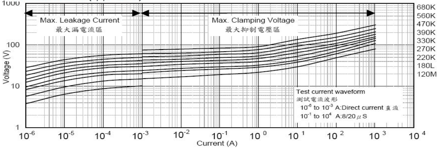
VDR-14D180L-14D680K(N/J/S SERIES)
