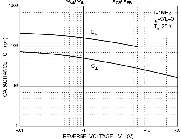
C_{cb}/C_{ib} - V_{CB}/V_{EB}
