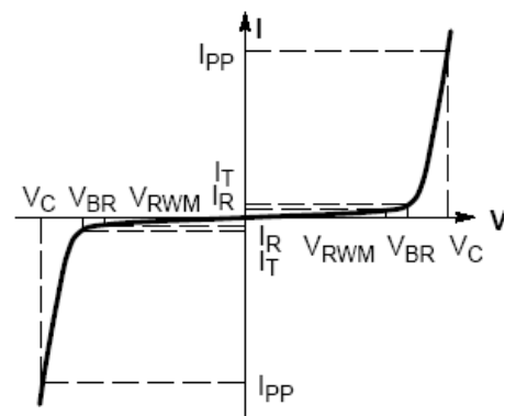
Bi-Directional TVS
