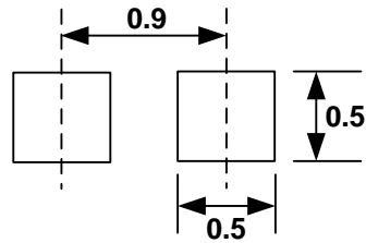
Soldering Footprint
