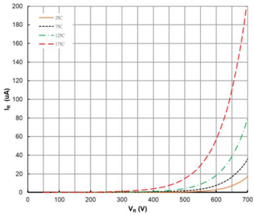
Figure 3. Reverse Characteristics
