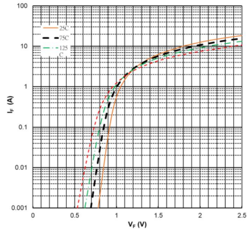
Figure 2. Forward Characteristics
