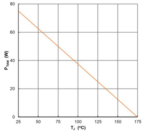
Figure 4. Power Derating
