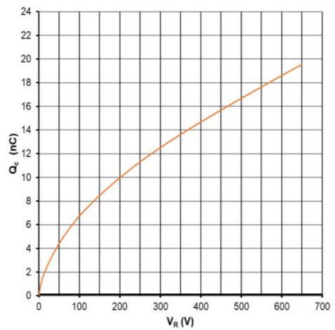
Figure 6. Recovery Charge vs Reverse Voltage
