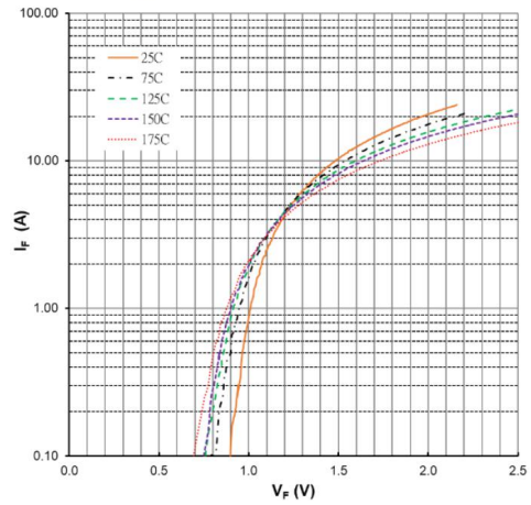
Figure 2. Forward Characteristics
