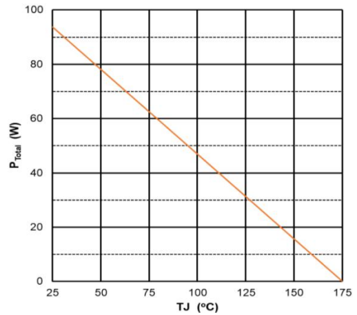
Figure 4. Power Derating
