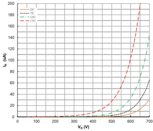
Figure 3. Reverse Characteristics
